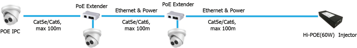
POE Extenders Cascade Deployment , powering 3 IP cameras over one Cat5E cable
