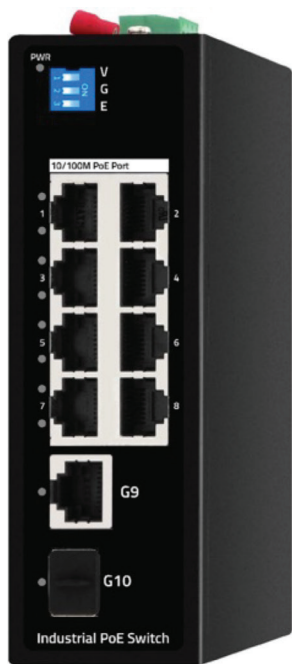
Preinstalled 8-Port 100Mbps and 1-Port Gigabit with 1-Port Gigabit SFP Industrial PoE Switch
