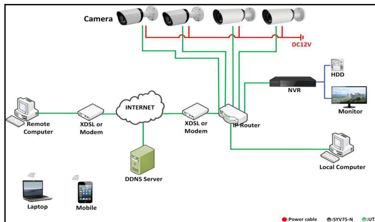
Network Connection
