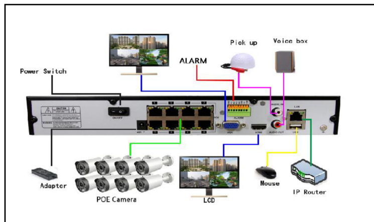
Device Connection
