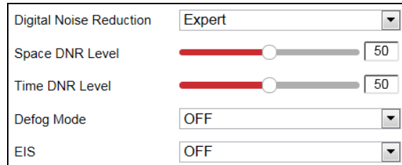
Figure 6-33 Expert Mode
