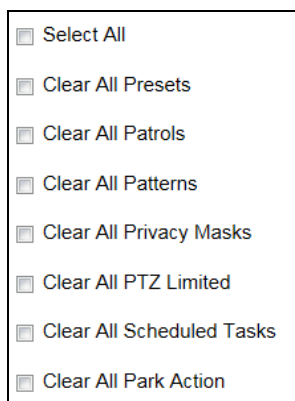
Figure 5-34 Clear Config
