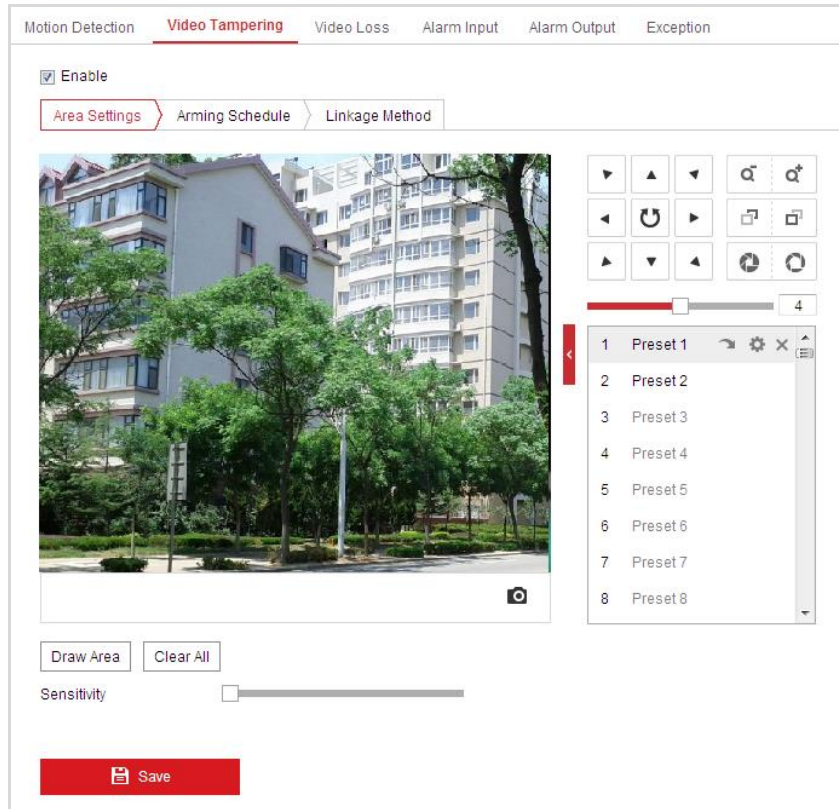
Figure 5-15 Tampering Alarm
