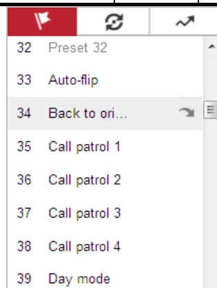
Figure 4-8 Special Preset
