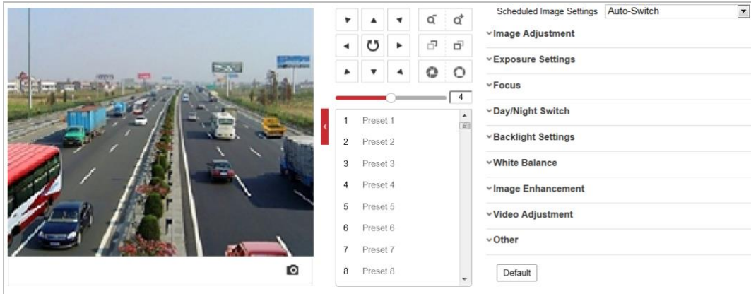
Figure 6-23 Display Settings
