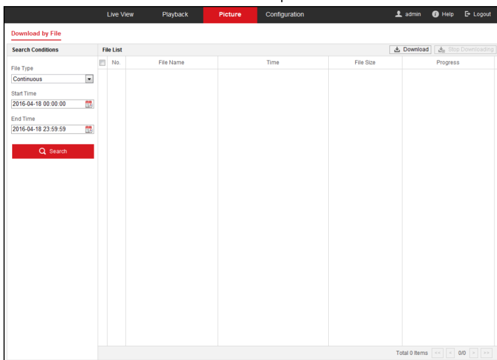
Figure 4-20 Picture Interface
